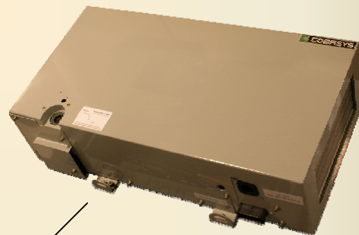
Model: NiMHax 144-30 ic with integrated cooling for interior installations
